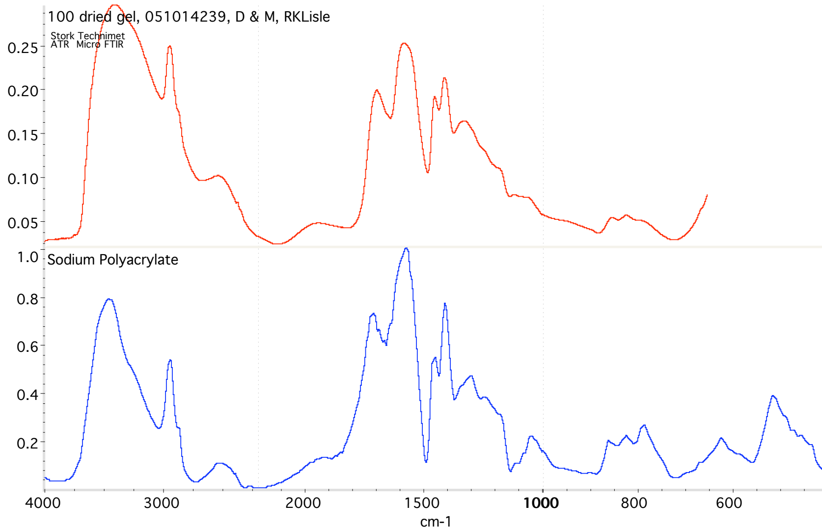
Figure 2 – Spectral Match of Dried Gel with Sodium Polyacrylate
